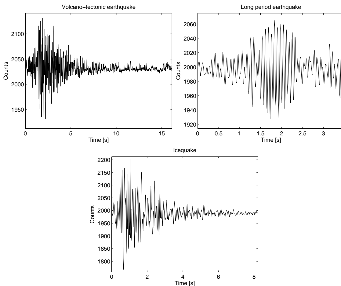
Figure 1. Typical waveforms of the three classes considered: VT, LP and IC events.
